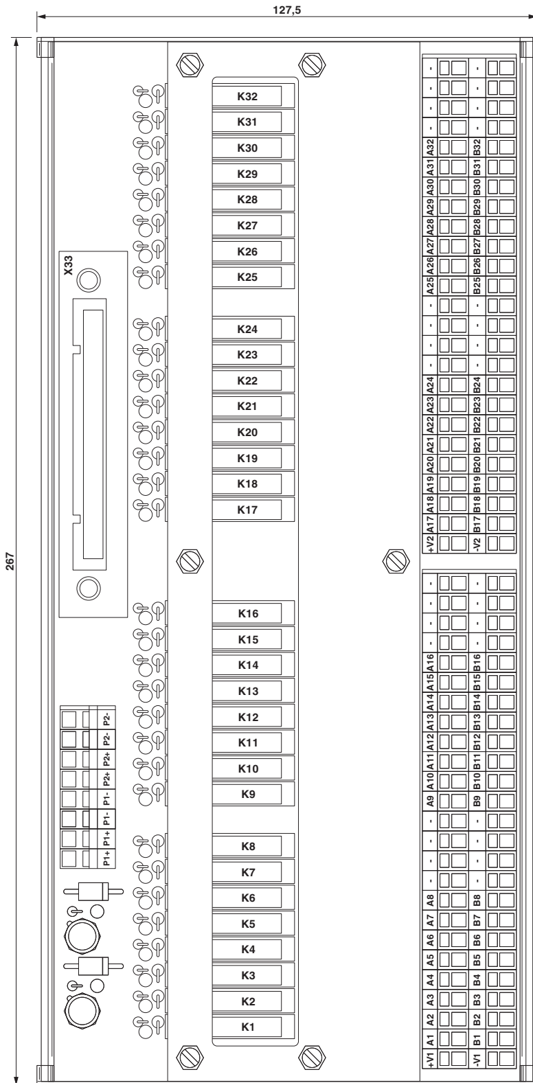
Dimensional drawing
